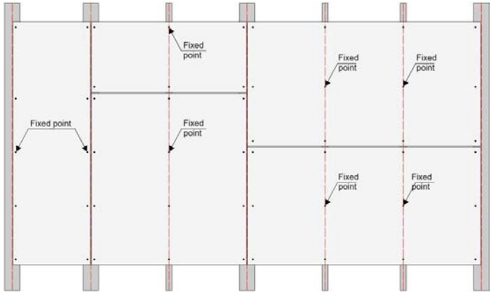
IMAGE 19- EXAMPLE OF CLADDING WITH KØL FIBRE CEMENT PANELS. IN SOME CASES, THE GEOMETRY OF THE PANEL AND THE FACADE LAYOUT MAY REQUIRE TWO FIXED POINTS.
