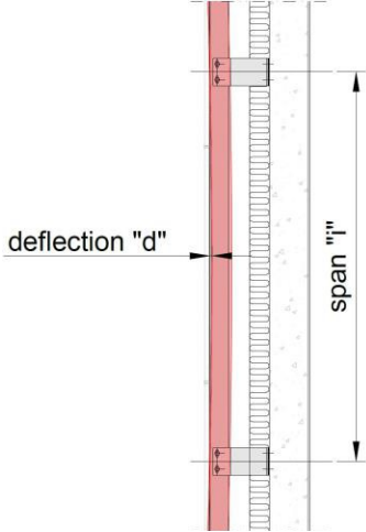
IMAGE 7 - THE MAXIMUM DEFLECTION OF THE BATTENS/PROFILES BETWEEN TWO BRACKETS d_{max} MUST BE \leq 1/200 FOR THE SPAN BETWEEN THE BRACKETS "l"
