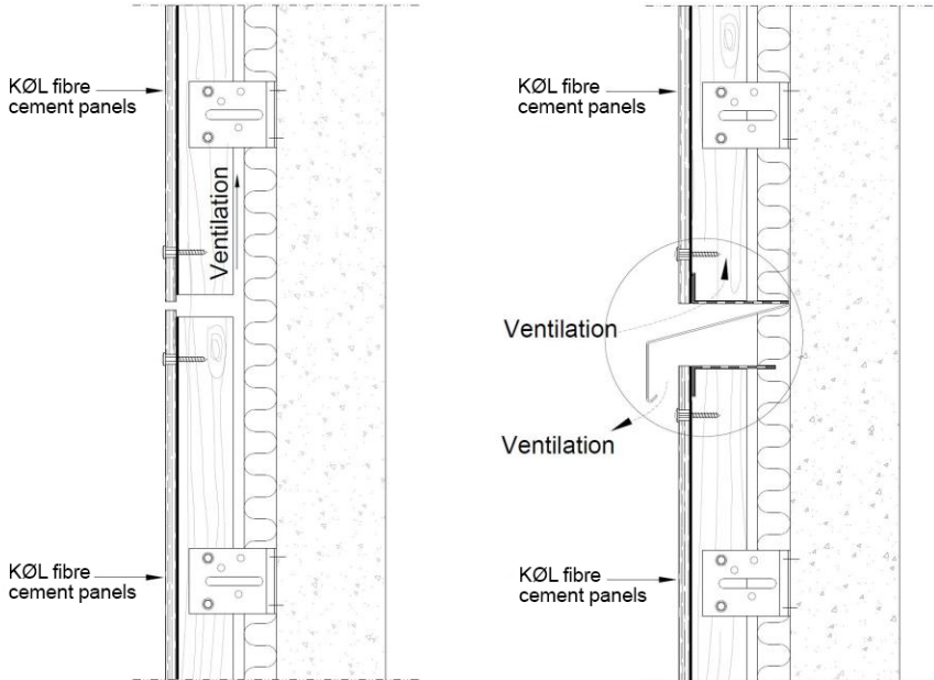
IMAGE 16 - EXAMPLE OF A CONTINUOUS AND PARTITIONED VENTILATED CAVITY ON A WOODEN SUBFRAME. THE FLASHINGS USED TO PARTITION THE AIR BARRIER MUST NEVER COMPROMISE THE FREE FLOW OF AIR. THE LAYER OF INSULATION MATERIAL IS OPTIONAL.
