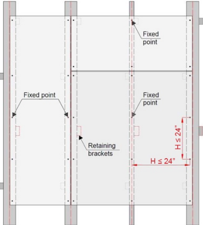
IMAGE 18 - EXAMPLE OF CLADDING WITH KØL FIBRE CEMENT PANELS. THE RETAINING BRACKET SHOWN IN RED SHOULD BE AS CLOSE AS POSSIBLE TO THE FIXED POINT OF THE PANEL.
