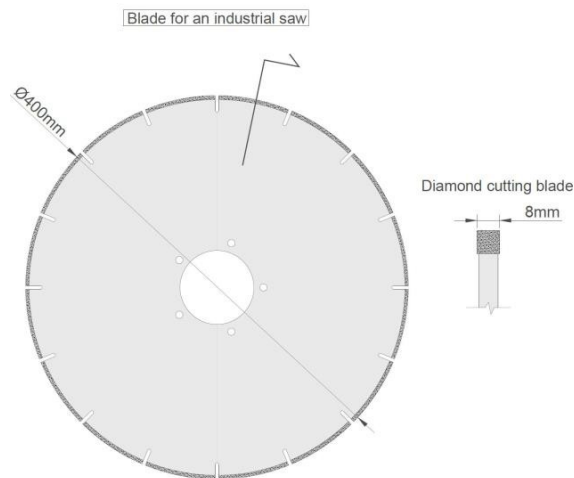
IMAGE 45 - EXAMPLE OF A BLADE USED TO CUT THE PANELS AT THE MANUFACTURER'S FACTORY
