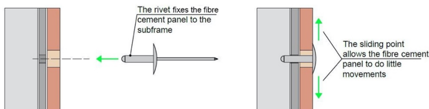
IMAGE 21 - EXAMPLE OF STEPS TO FIX KØL FIBRE CEMENT PANELS. THE PANELS ARE PRE-DRILLED WITH HOLES THAT ALL HAVE THE SAME DIAMETER OF 9.5 MM (3/8"). THE EXAMPLE SHOWS HOW THE DIAMETERS OF THE HOLES FOR THE FIXED POINTS ARE REDUCED USING SUITABLE METAL BUSHINGS.
