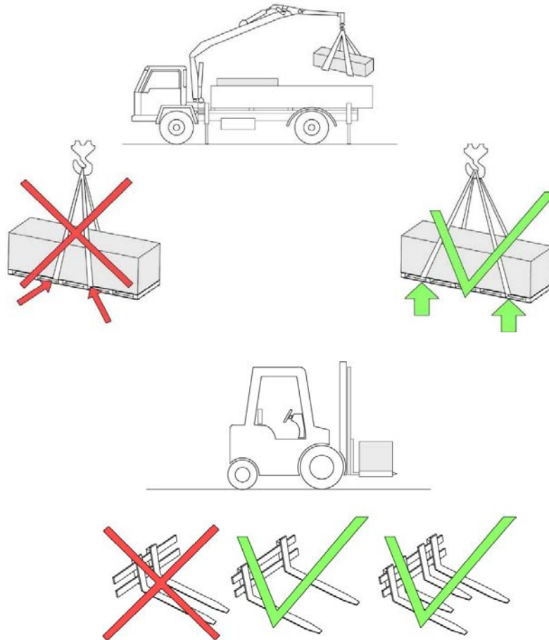
IMAGE 39 - TRANSPORT AND HANDLING OF PANELS
