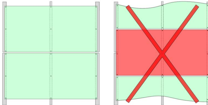
IMAGE 23 – LEFT: EXAMPLE OF A CORRECT WAY TO SECURE KØL PANELS, WITH THE HORIZONTAL JOINT OF THE CLADDING ALIGNING WITH THE EXPANSION JOINT OF THE SUBFRAME PROFILES. RIGHT: EXAMPLE OF AN INCORRECT WAY TO SECURE THE KØL PANELS, WITH A CLADDING SHEET SECURED TO TWO PROFILES.
