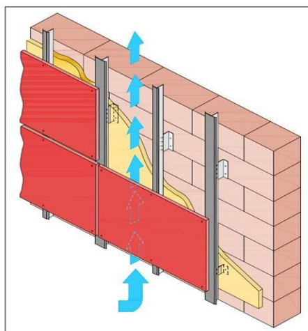
IMAGE 2 - EXAMPLE OF SUBFRAME WITH METAL PROFILES AND BRACKETS. THIS LAYING CONFIGURATION INCLUDES A LAYER OF THERMAL INSULATION (OPTIONAL). THE ARROWS SHOW THE FLOW OF AIR CIRCULATING IN THE VENTILATED CAVITY.
